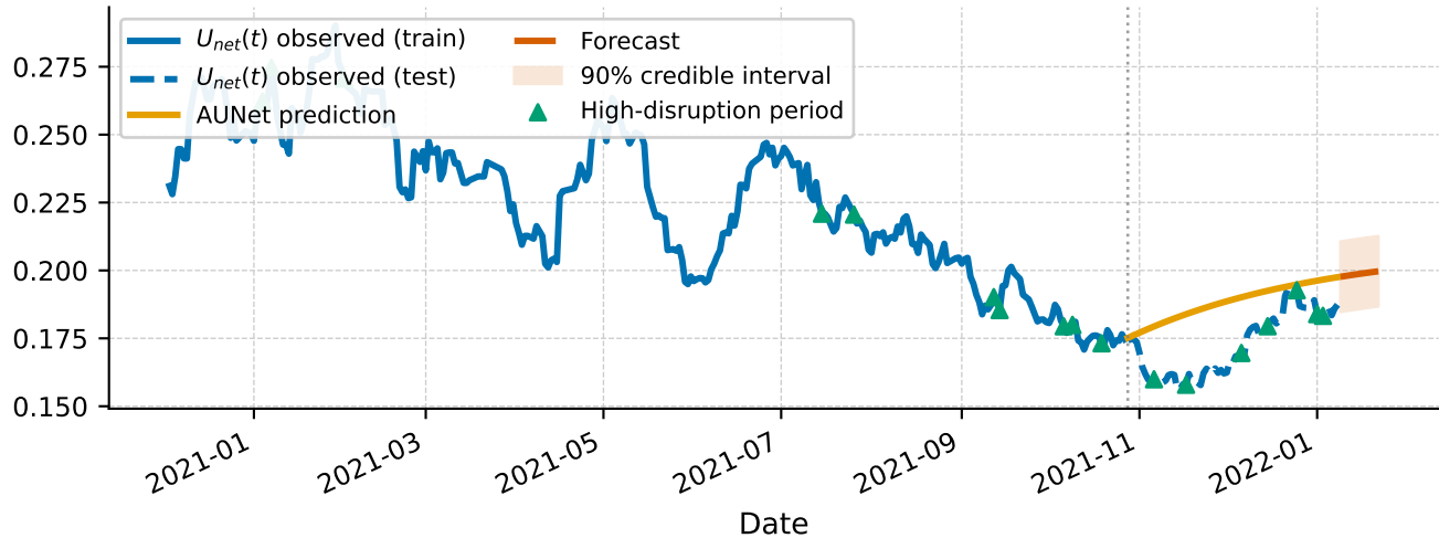
AUNet Network-Level Uncertainty Trajectory
